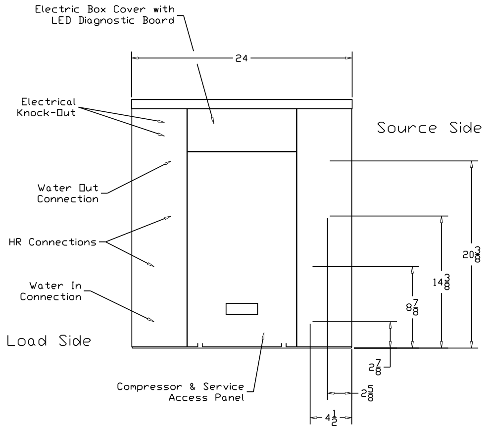
Front Elevation
